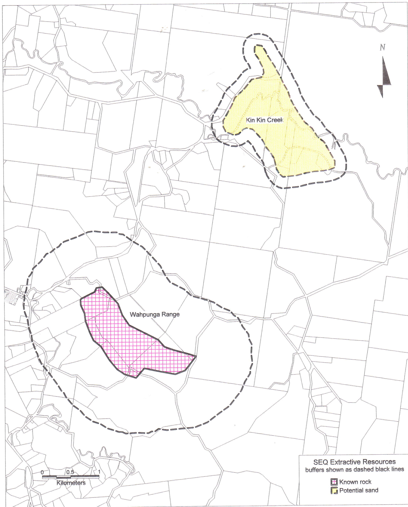
Figure 8. Hardrock and sand resources in the Wahpunga Range - Kin Kin Creek area, Noosa Shire
